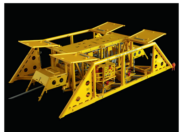
TRYM bunnramme – Dong Energy
